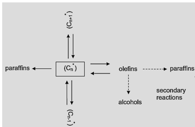
Fig. 5. Illustration of chain growth and termination parameters in the Fischer-Tropsch synthesis [10].
