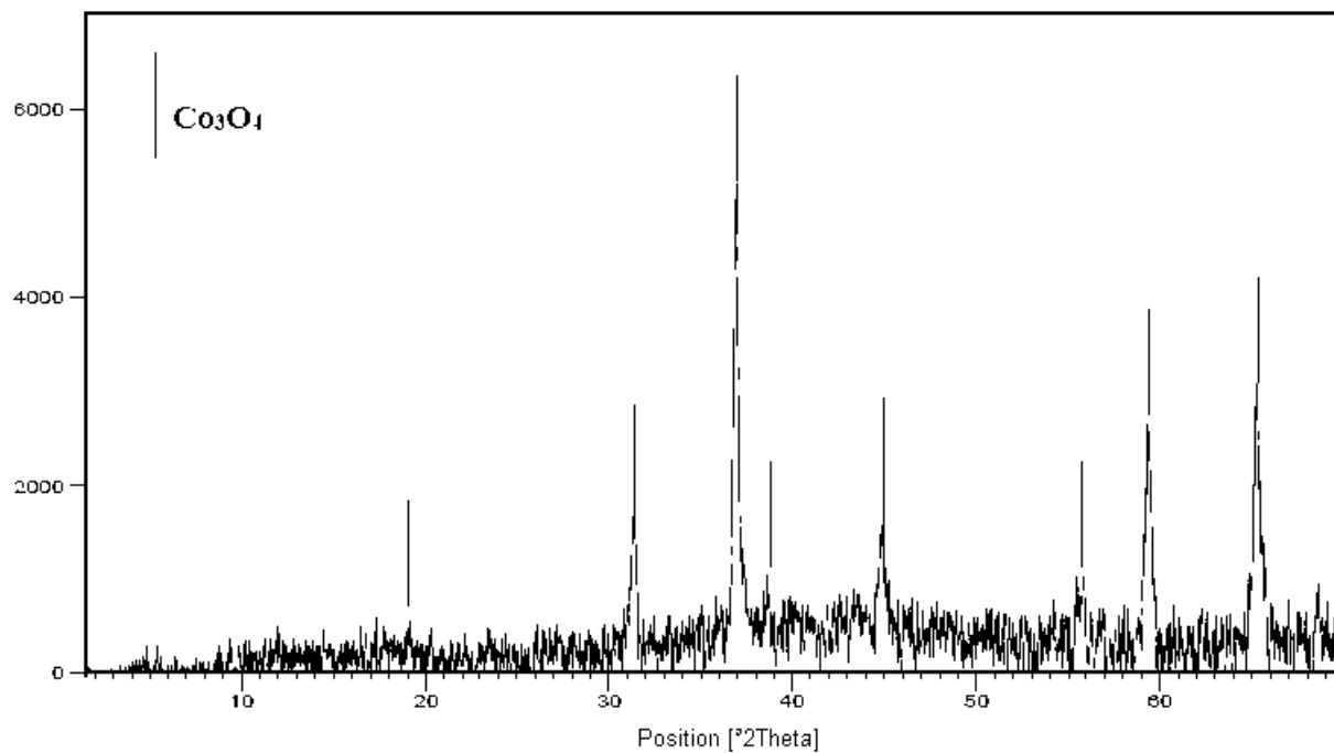
Fig. 2. XRD pattern of calcined \text{Co}/\text{Al}_2\text{O}_3 catalyst.
