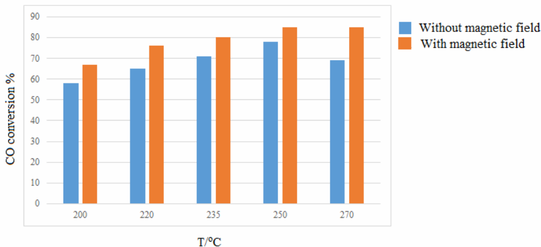
Fig. 6. The CO conversion (%) as a function of reaction temperature in FT reaction on Co/Al 2 O 3 catalyst without and with external magnetic field (1 atom, H 2 /CO = 2, 3500 h -1 ).
