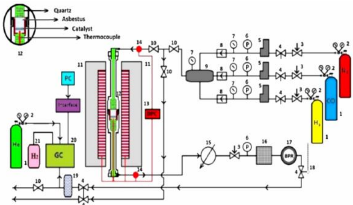
Fig. 1. Schematic of reactor for FT reaction, 1-gas cylinders, 2-pressure regulators, 3-needle valves, 4-simple valves, 5-mass flow controllers, 6-digital pressure gauges, 7-pressure gauges, 8-one-way valve, 9-mixing chamber, 10-ball valve, 11-furnace, 12-reaction zone, 13-temperature controller, 14-resistant temperature detector, 15-exchanger, 16-liquid trap, 17-back pressure regulator, 18-flow meter, dewetter, gas chromatograph, hydrogen generator.
