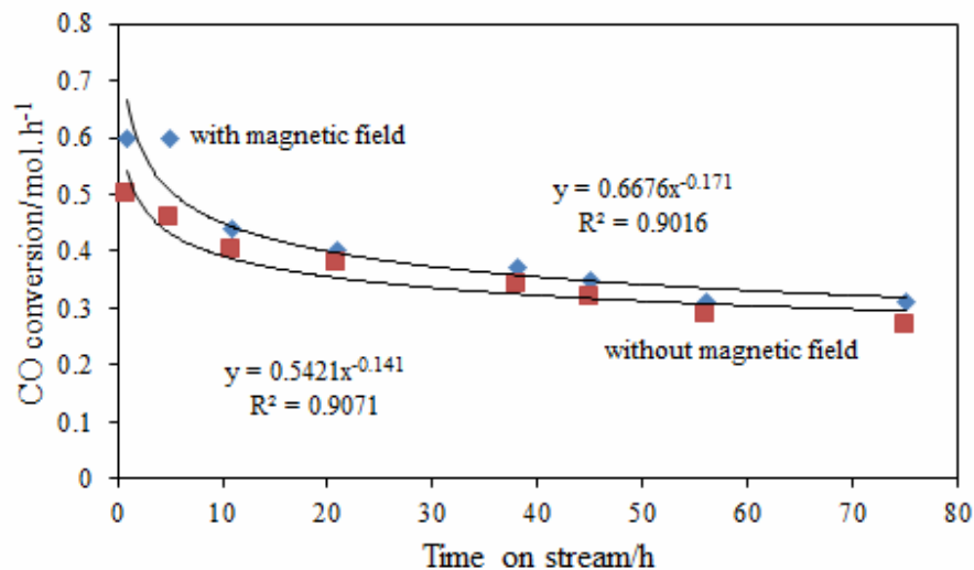
Fig. 8. The effect of magnetic field on the deactivation process after 75 h in the FT reaction at 230 °C, 1 bar, H 2 :CO = 2:1, GHSV = 1500 h -1 .
