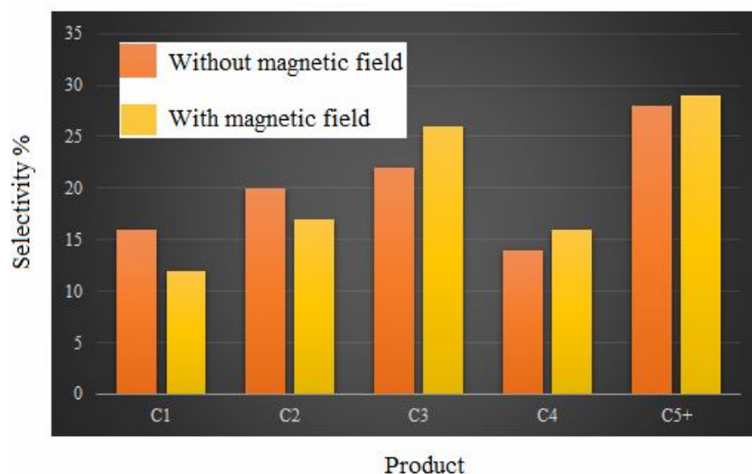
Fig. 7. A comparison of the product selectivity obtained from FT reaction on Co/Al 2 O 3 catalyst without and with external magnetic field.
